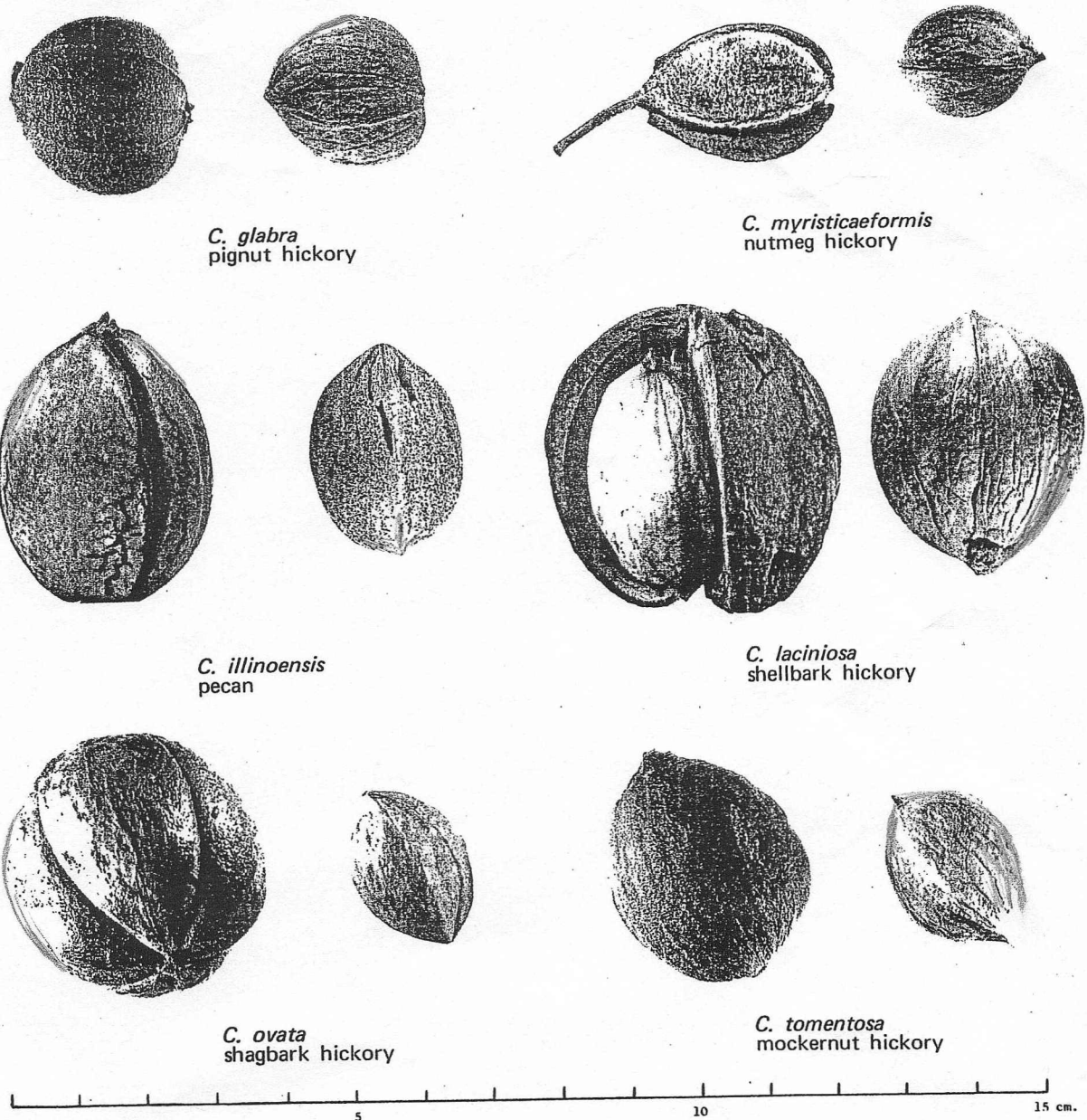
Figure 1. Carya : hickory nuts with husks attached and removed ( \times 1 ). Size and shape of the nuts may vary greatly within each species and may differ from the examples shown here (Bonner and Maisenhelder 1974a).
